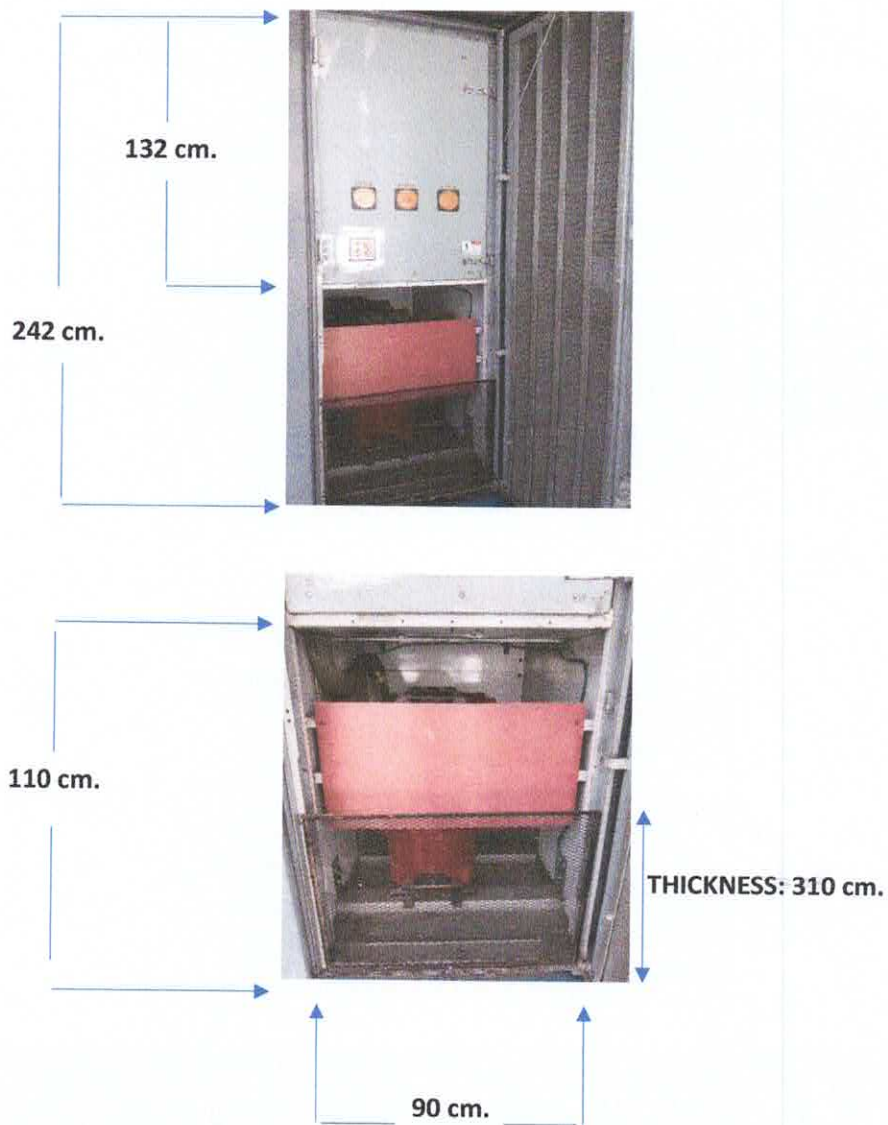
Existing Power Transformer 100KVA
